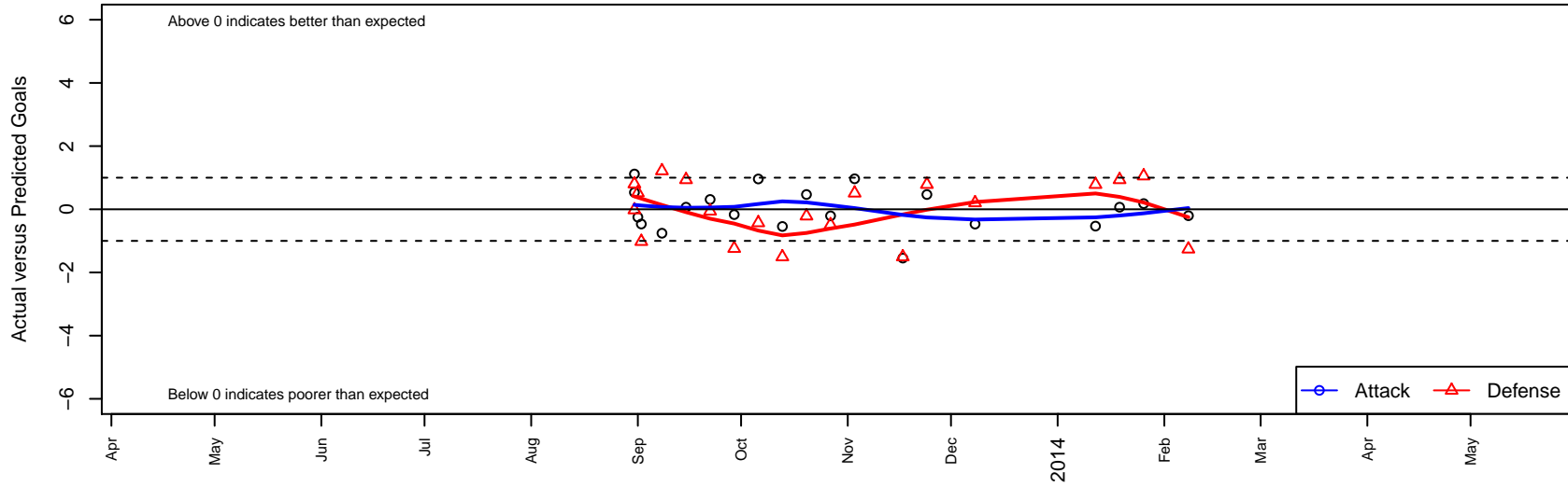
LVR Freedom B96 Dots are actual minus expected GF (blue circles) and GA (red triangles). Blue line is smoothed change in attack strength. Red is smoothed change in defense strength.
